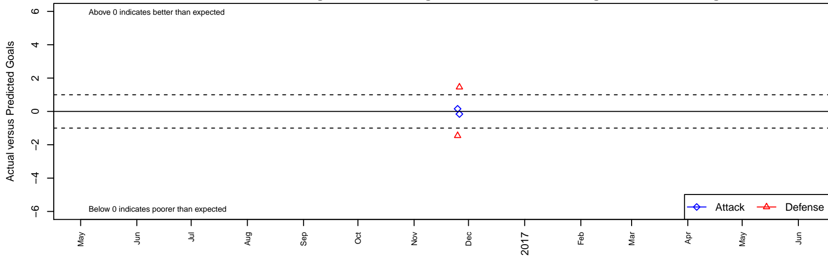
SAC Premier Blue B98 Dots are actual minus expected GF (blue circles) and GA (red triangles). Blue line is smoothed change in attack strength. Red is smoothed change in defense strength.
